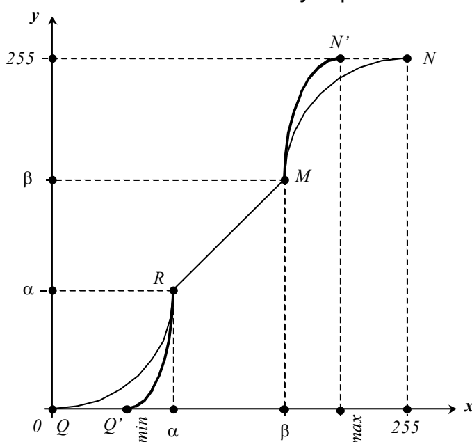
Fig. 3. Graph of transformation function in the interval [0, 255]
